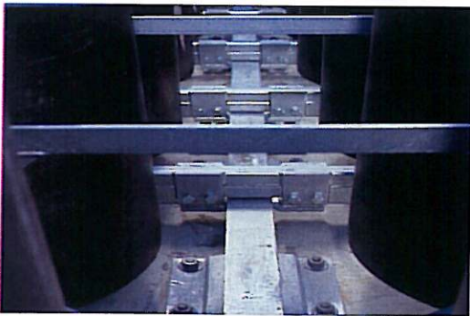
The REACT 350 System uses a monorail to provide lateral strength.
