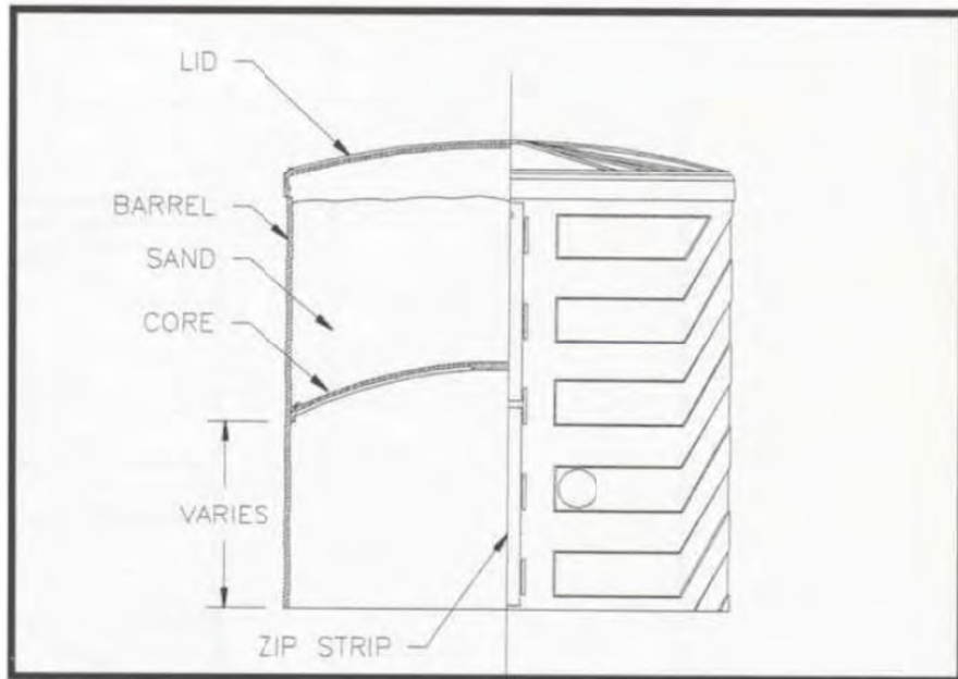
Figure 1C-Fitch® Universal Module System
